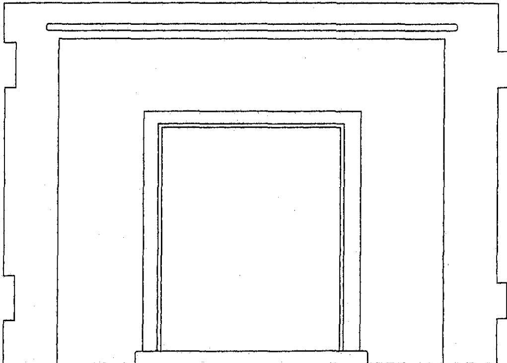
Part No. 300 Loading/Double Entry Dorr Wall Section (2)
